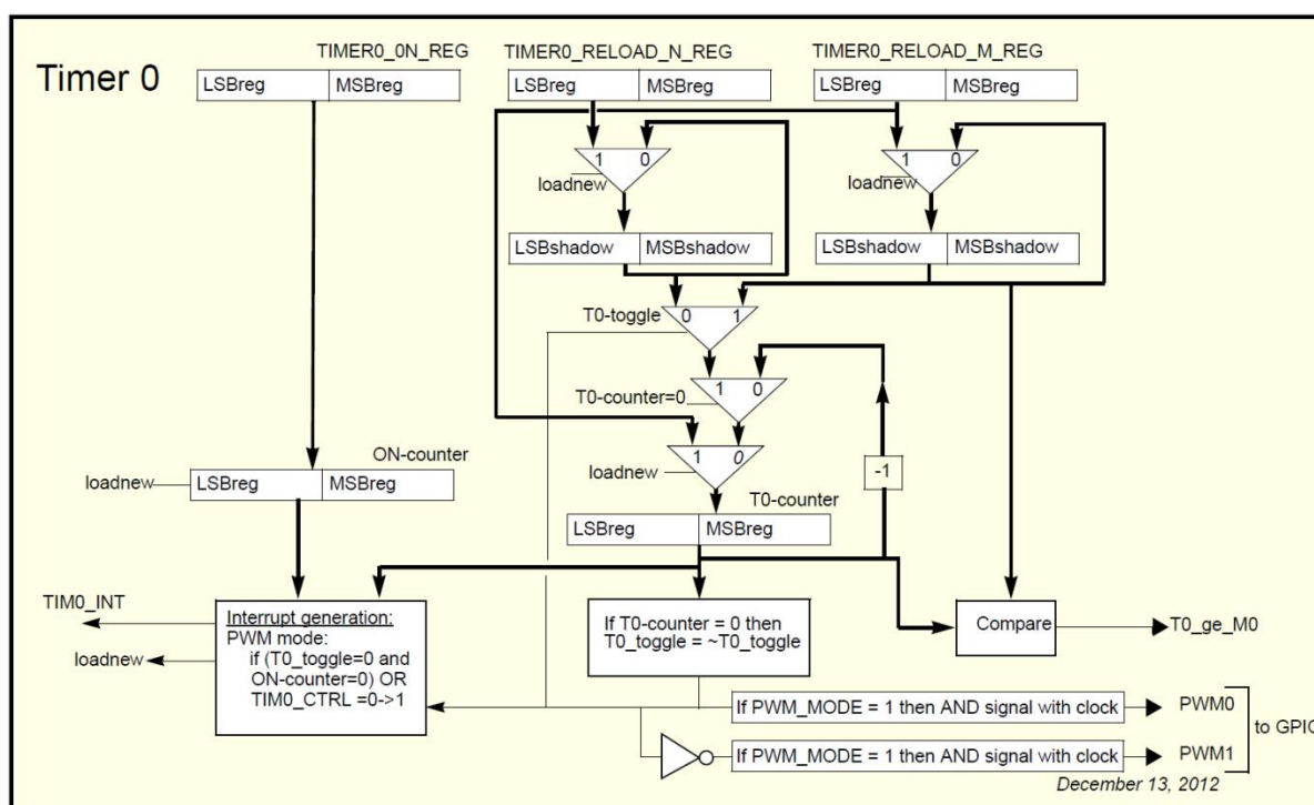
Figure 57: Timer 0 Block Diagram
