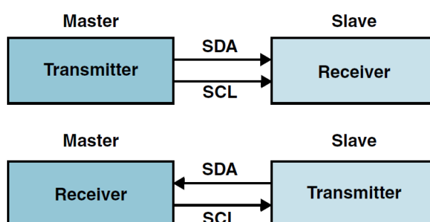
Figure 33: Master/Slave and Transmitter/Receiver Relationships
