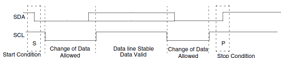
Figure 35: START and STOP Conditions
