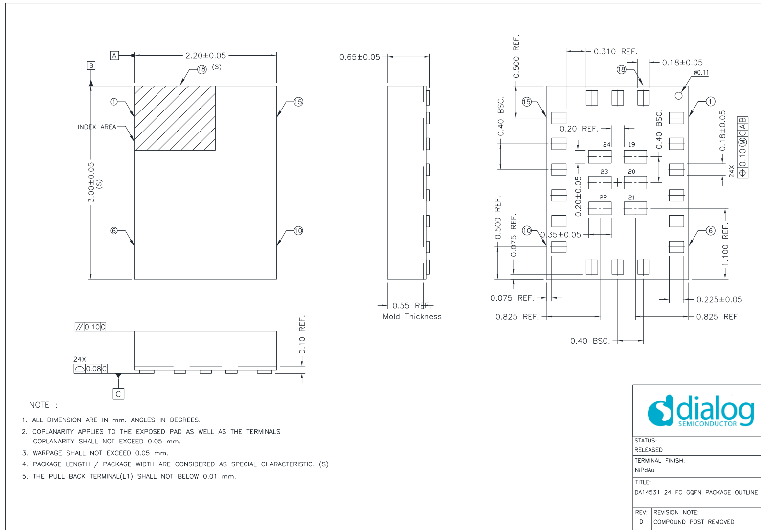
Figure 85: FCGQFN24 Package Outline Drawing
